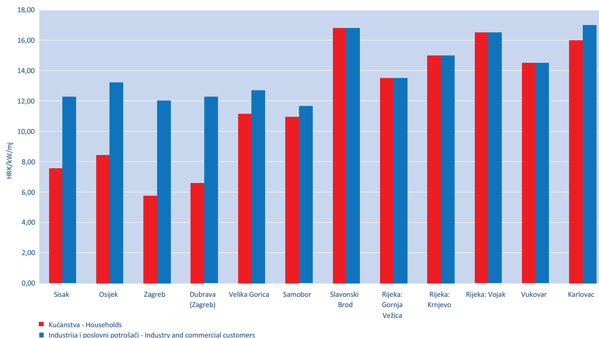
Slika | Figure 6.4.2. Usporedba tarifnih stavki pojedinih toplinarskih tvrtki za tarifni element zakupljene snage, po kategorijama kupaca (bez PDV-a), na kraju 2014. | Comparison of tariff items (without tax) for capacity by customer categories for central Dh systems of district heating companies, monthly cost, at the end of 2014 – Izvor | Source: EIHP
